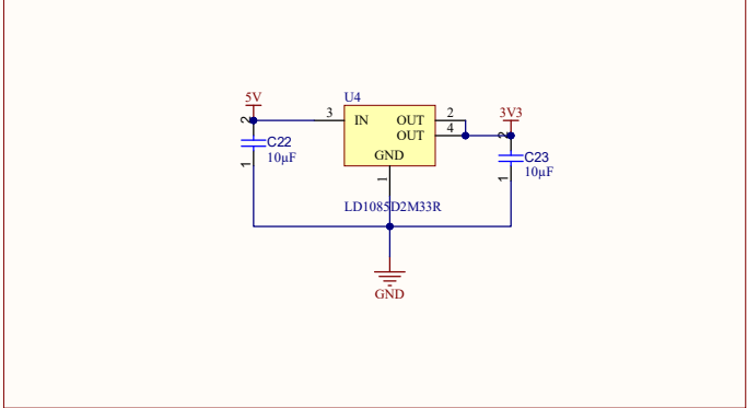
Fixed 3.3V Power Stage
