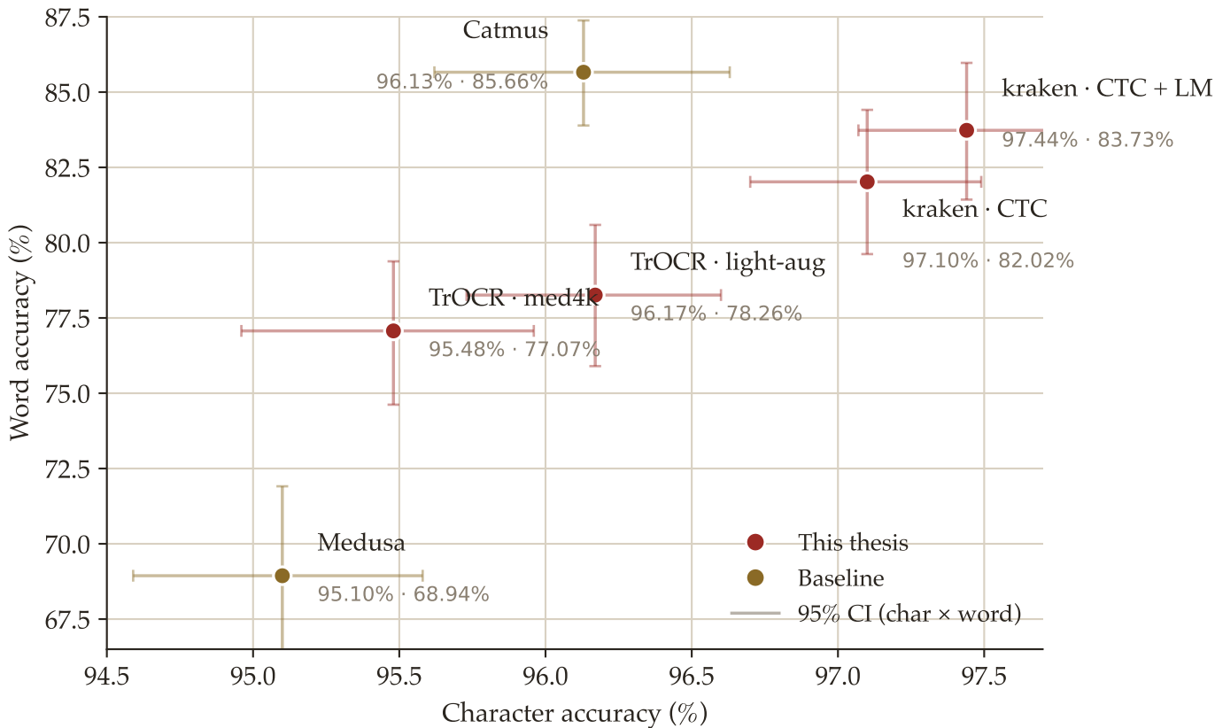
AlbucE OCR — accuracy trade-off (300-line validation, 95% CI)
