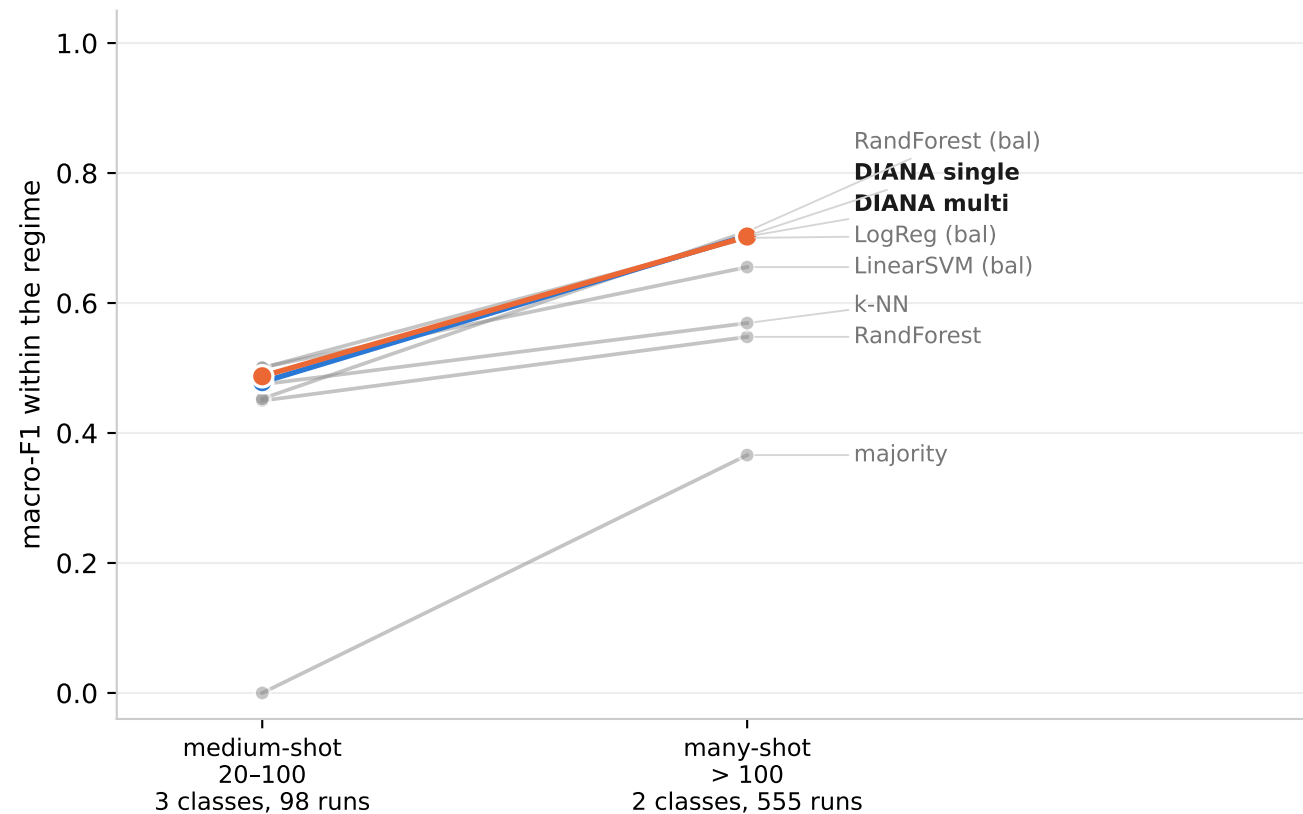
Held-out macro-F1 by training support — community_type
