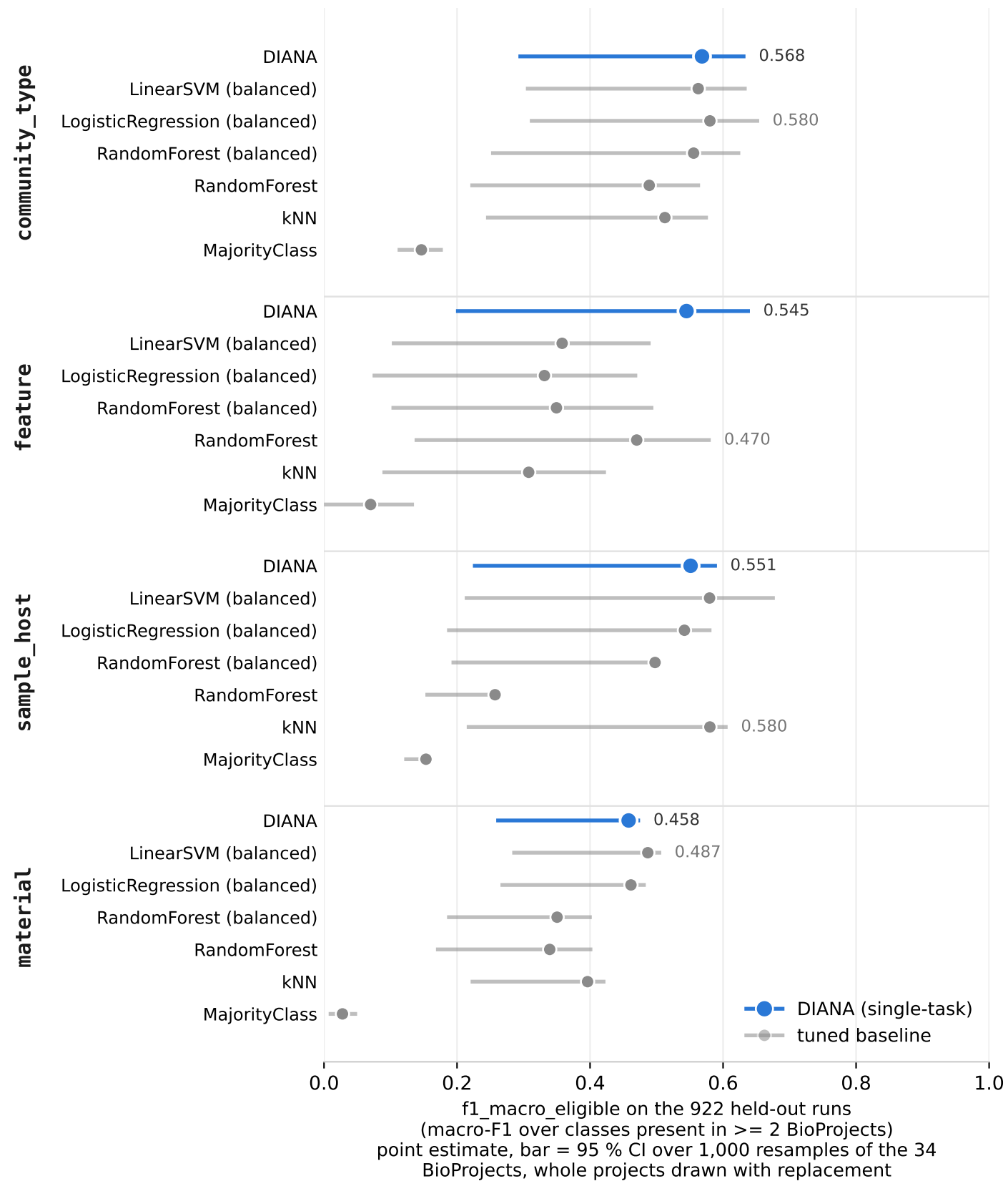
Held-out f1_macro_eligible by task and model
