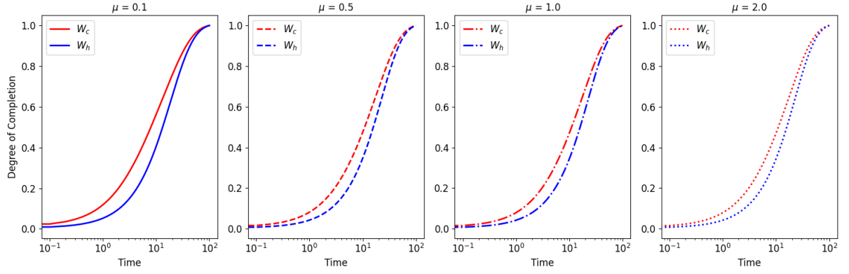
Figure 12 – Degree of completion for a displaced thermal state. Each graph corresponds to a different displacement parameter ( \mu ).
