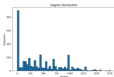
Figure 2: Degree distribution.
