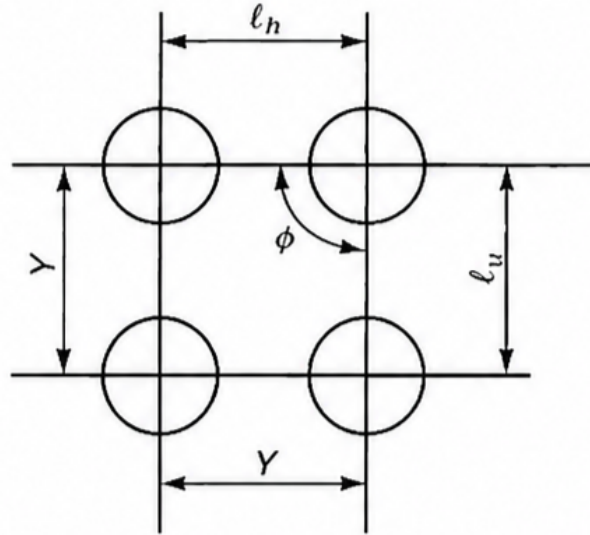
Figure 7.5: Selected tube array.
