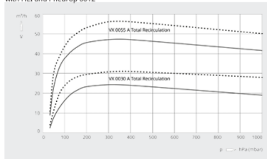
Pumping speed Dry air at 20 °C. Operating fluid water 15°C. Tolerance: - 10%, in accordance with HEI and Pneurop 6612
