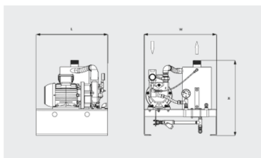
Dimensional drawing
