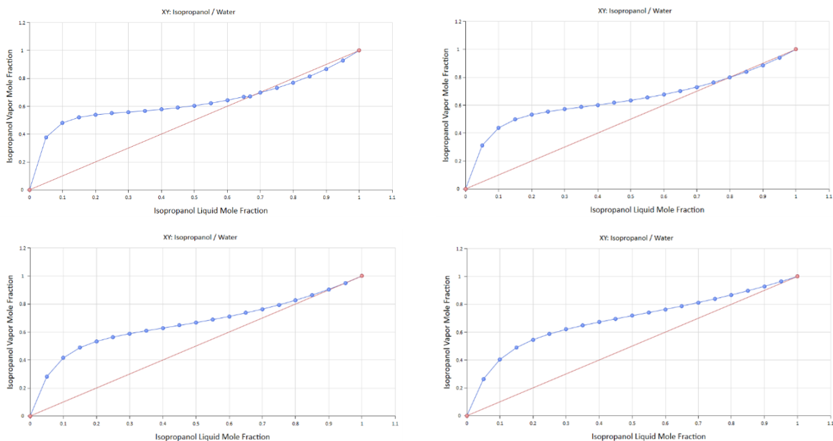
Figure 3.2: Effect of the DMSO concentration in the charge composition on the azeotrope, at 0.01, 0.05, 0.1 and 0.2 mole fraction, respectively.
