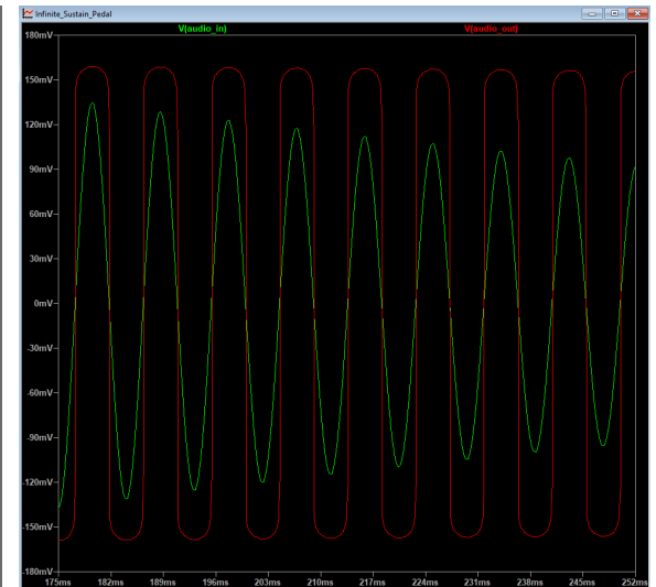
LT Spice [Input → Green, Output → Red]
