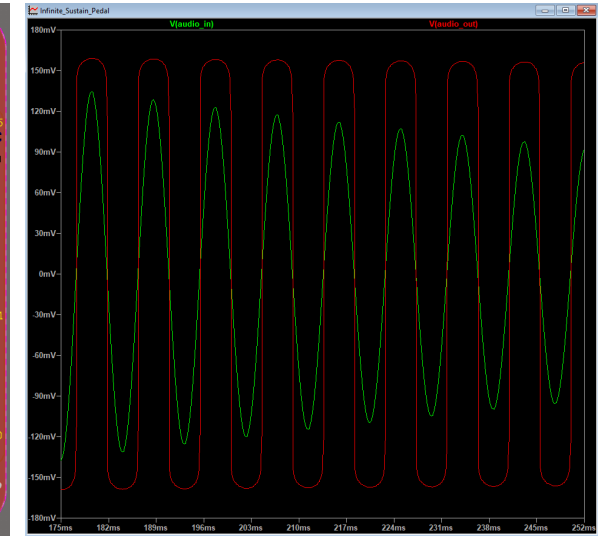
LT Spice Simulation [Input → Green, Output → Red]
