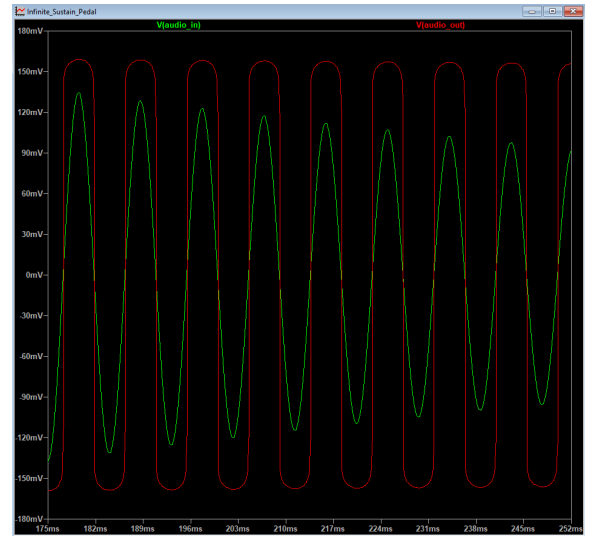
LT Spice Simulation [Input → Green, Output → Red]
