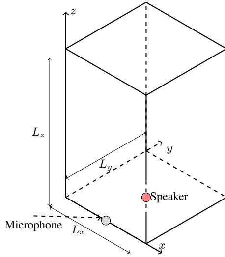
FIG. 1(b): Detailed positions of microphone and speaker within the rectangular cavity (3-D view)
