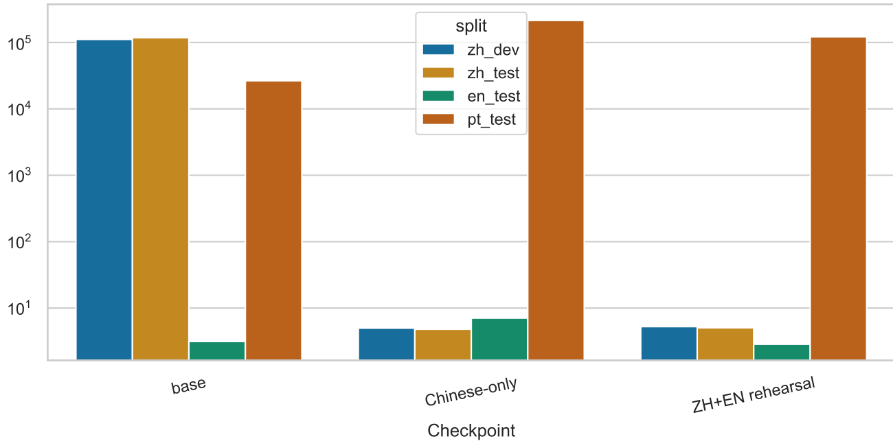
Perplexity (log scale)
