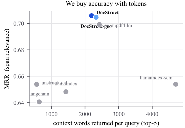
Figure 5: Accuracy against the token bill. DOCSTRUCT sits top-centre: best MRR, but roughly four times the context of unstructured and langchain, which sit bottom-left. A deployment that pays per token may reasonably prefer the bottom-left corner.
