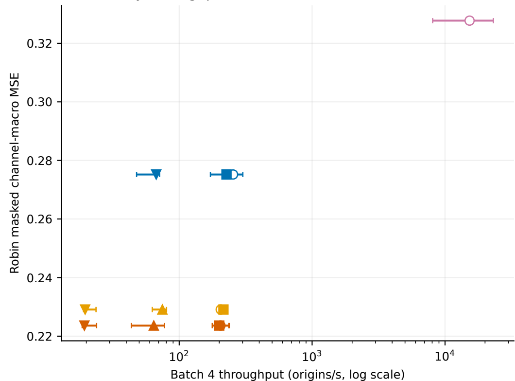
B Accuracy-throughput
