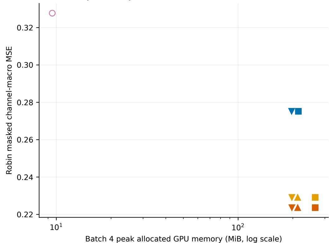
A Accuracy-memory
