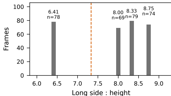
(c) Slenderness over frames (KS 7.33)
