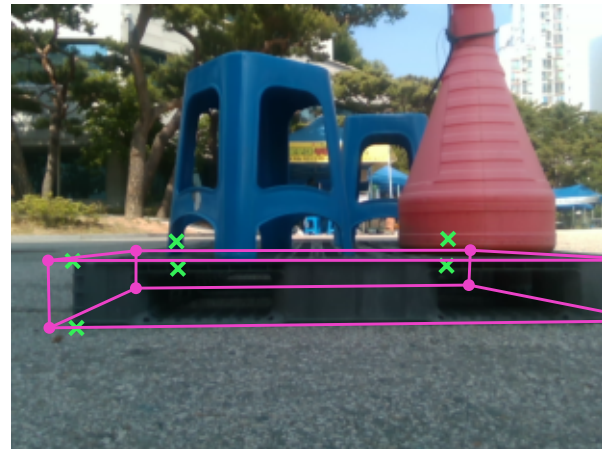
Corrected-pseudo student mean scored error 34.75px
