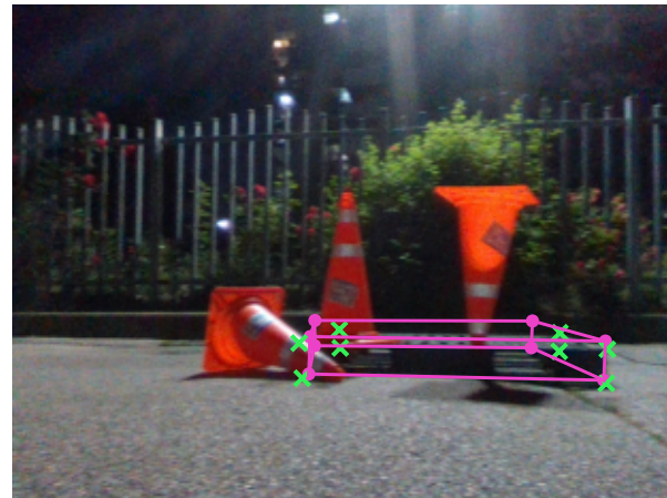
Corrected-pseudo student mean scored error 17.34px
