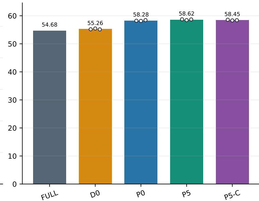
ALL-GT PCK10 (%) ↑
