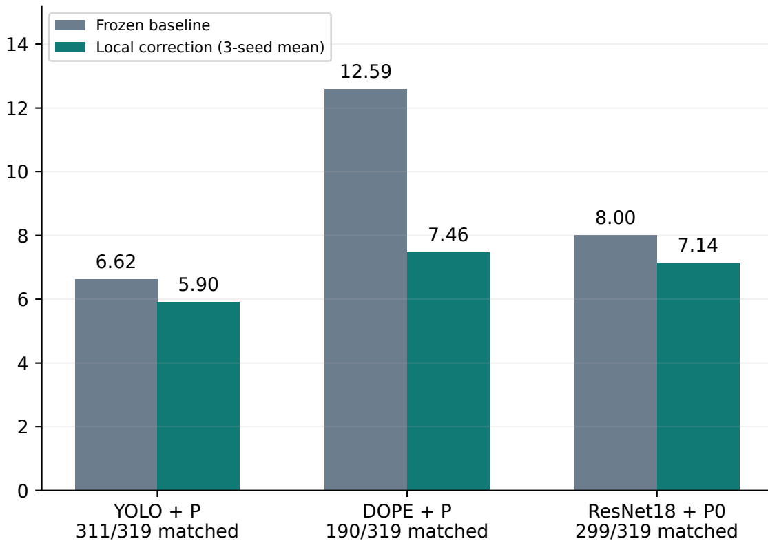
Conditional 2D median (px, lower better)
