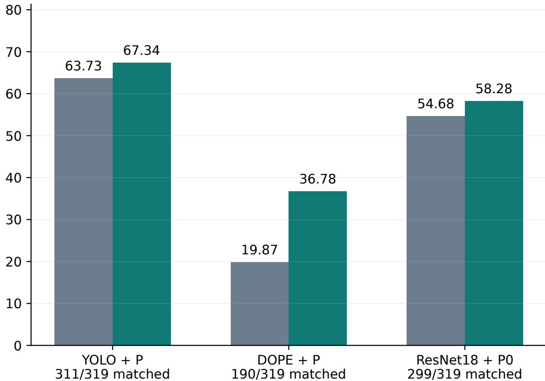
All-GT PCK10 (% , higher better)
