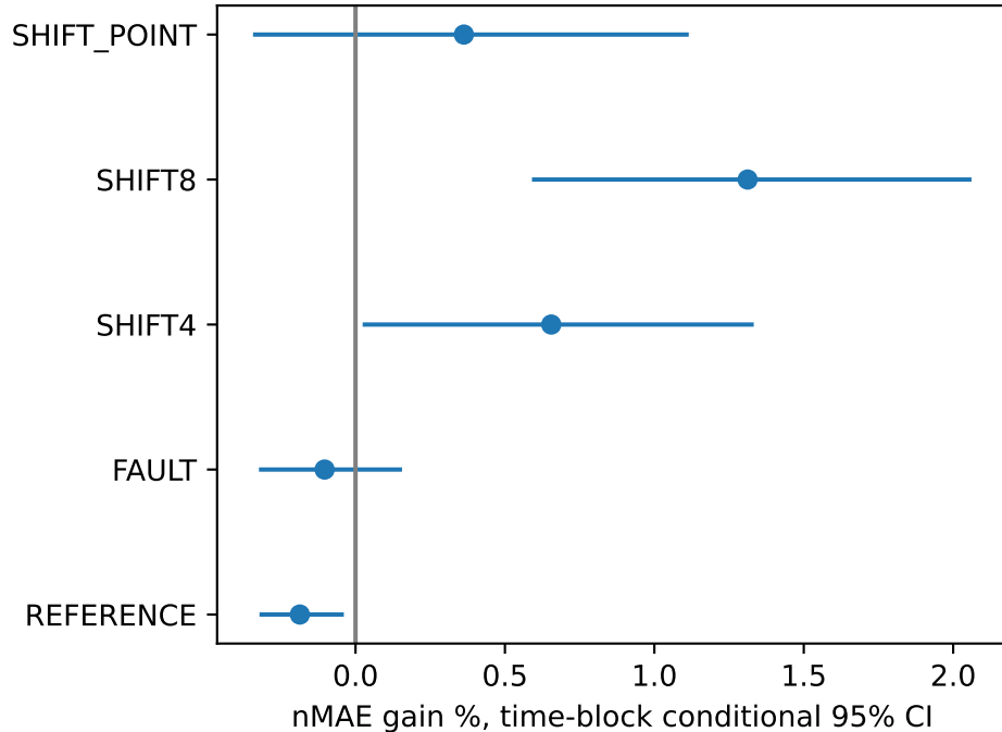
NESO2025: C3 vs C2
