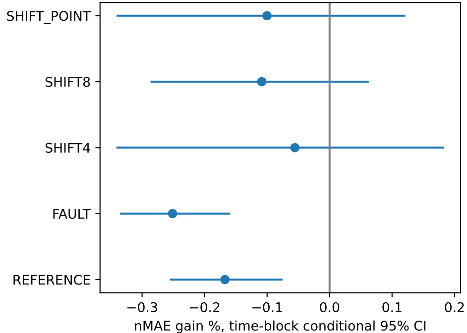
NESO2025: C3 vs M_RECENCY
