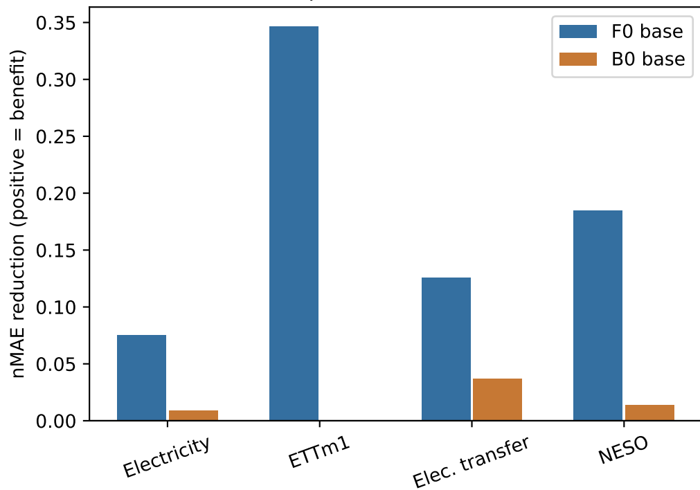
Total adapter benefit vs own base
