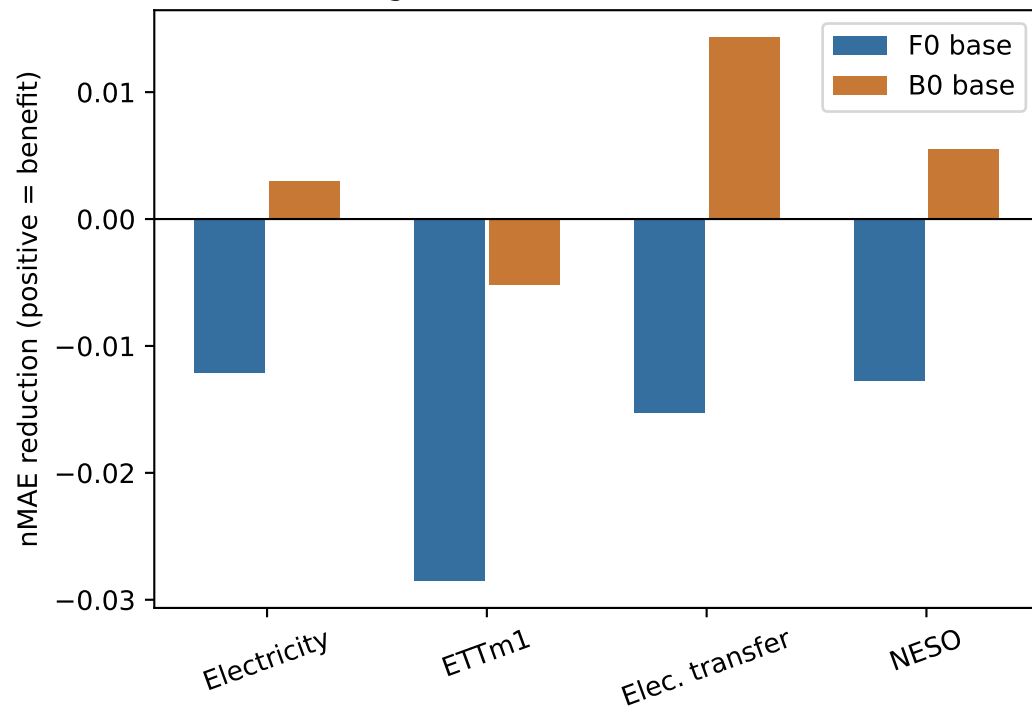
Magnitude-rule benefit vs PLAIN
