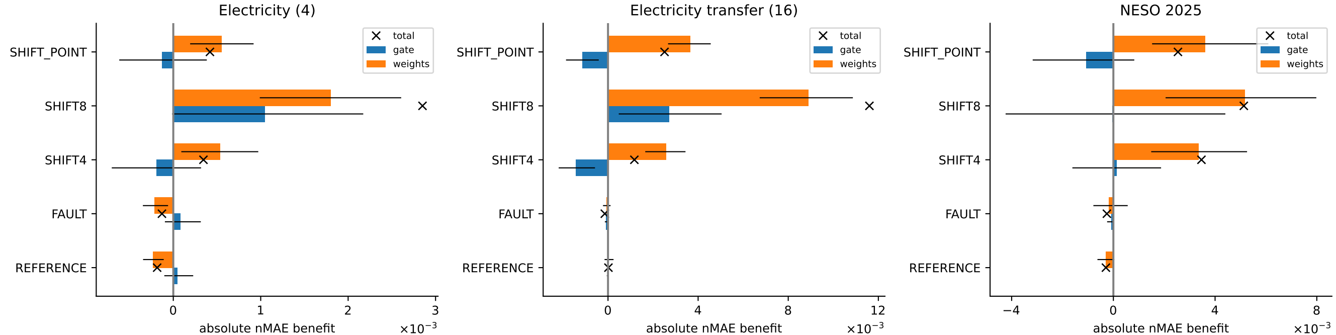
C3 vs C2: matched LR and 1024 updates; inference gate and learned-weight contrasts
