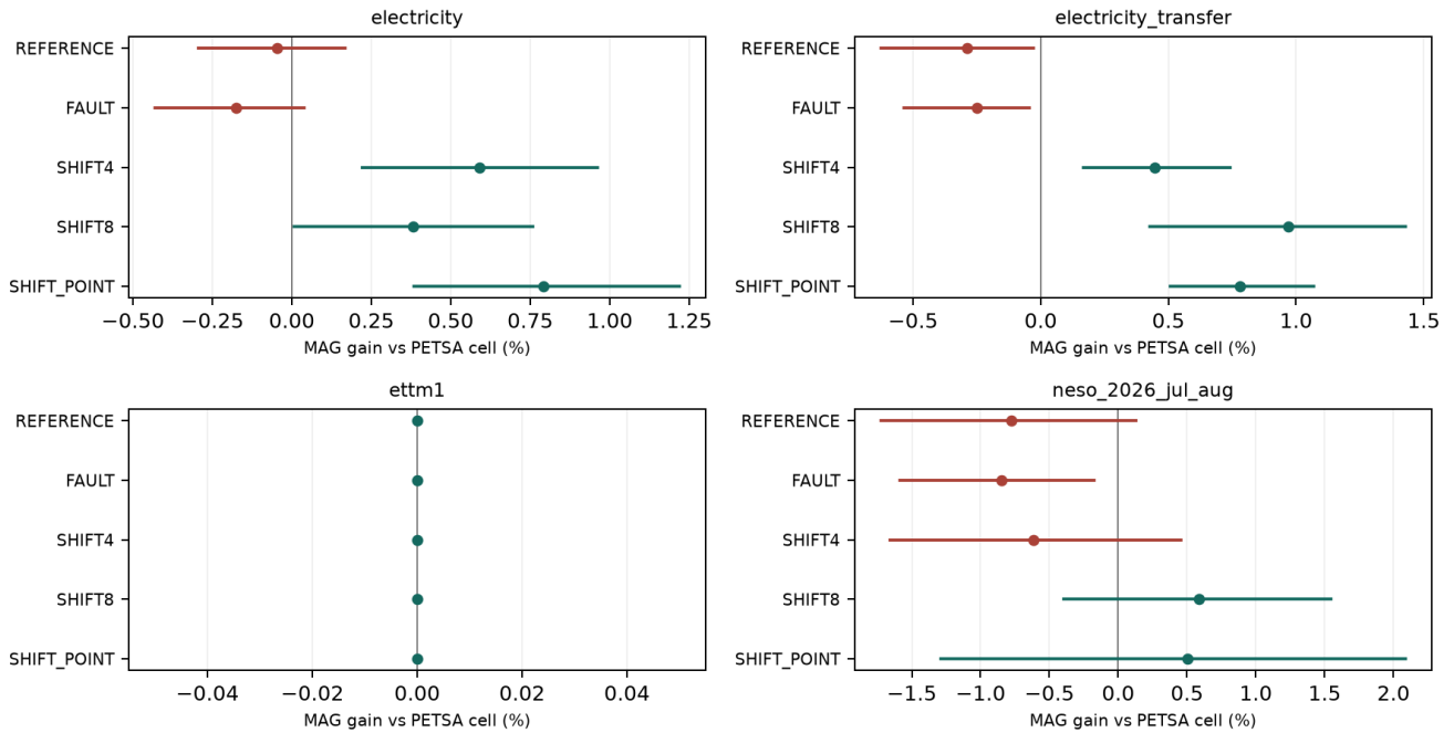
Offline controlled transfer: all reused development panels; marginal 95% intervals
