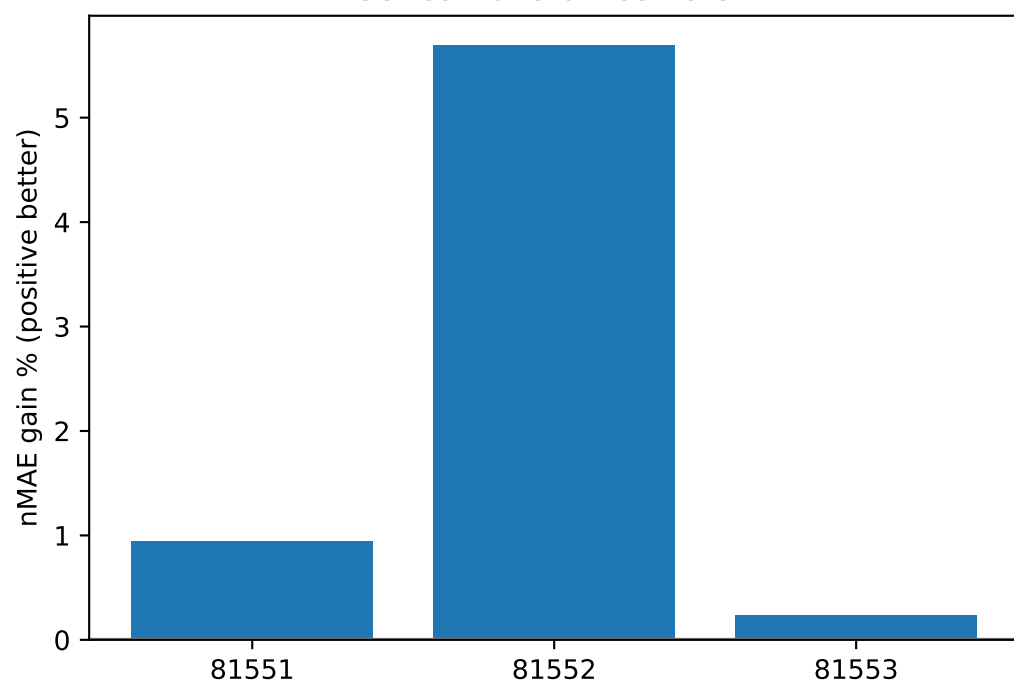
Series transfer: C3 vs C2
