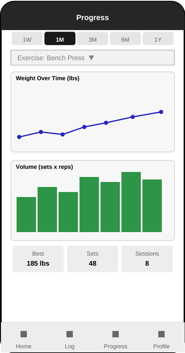
Screen 3: Progress
