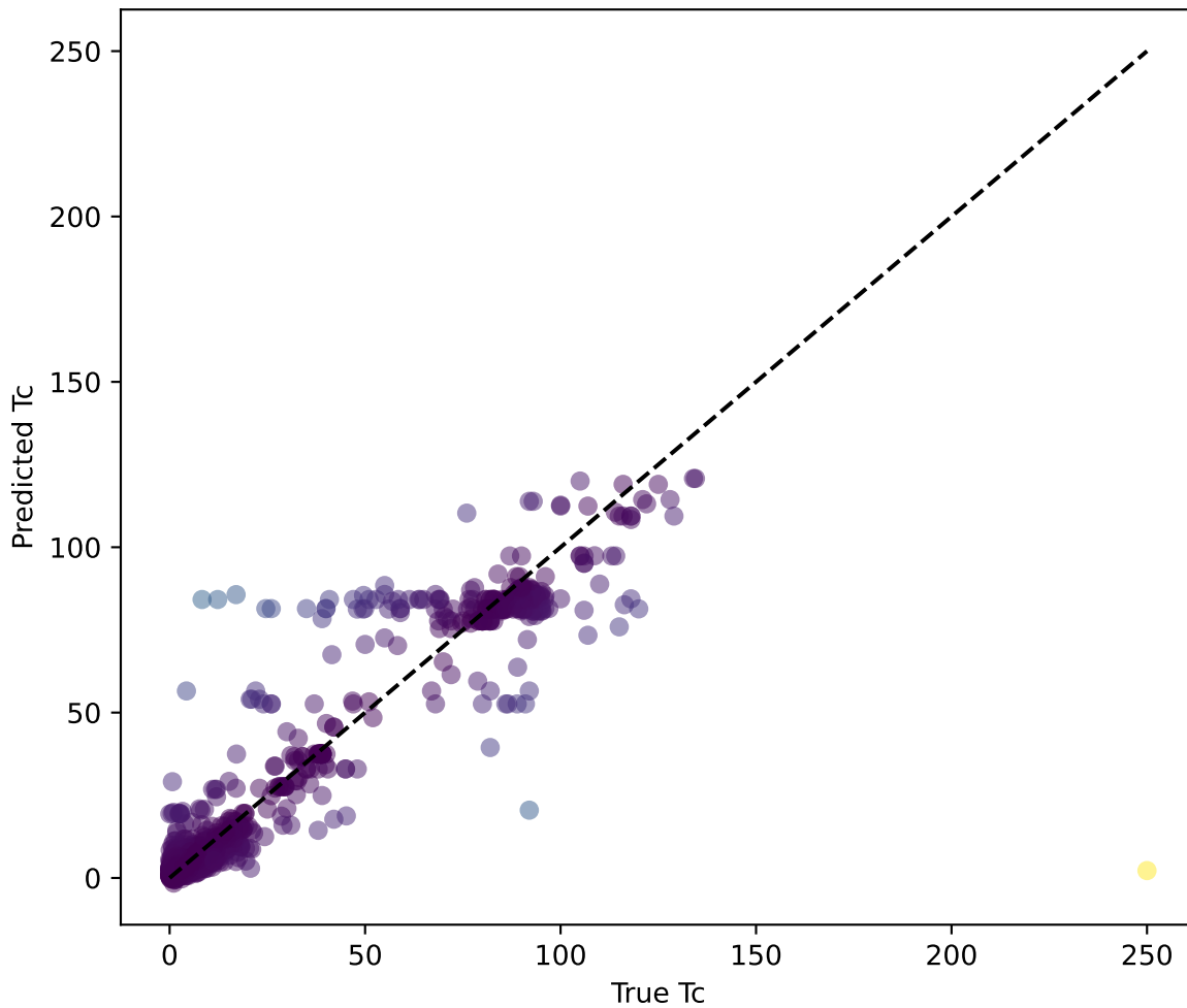
Prediction Analysis ( R^2=0.889 )
