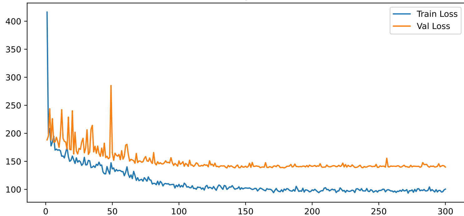
Training Curve
