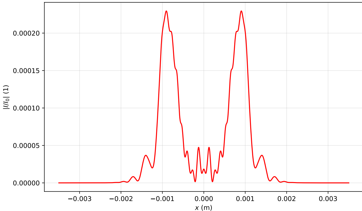
Intensity profile I(x, y = 0, z = 0.637)/I_0 , P_{in}=11.0P_{cr} , artificial time
