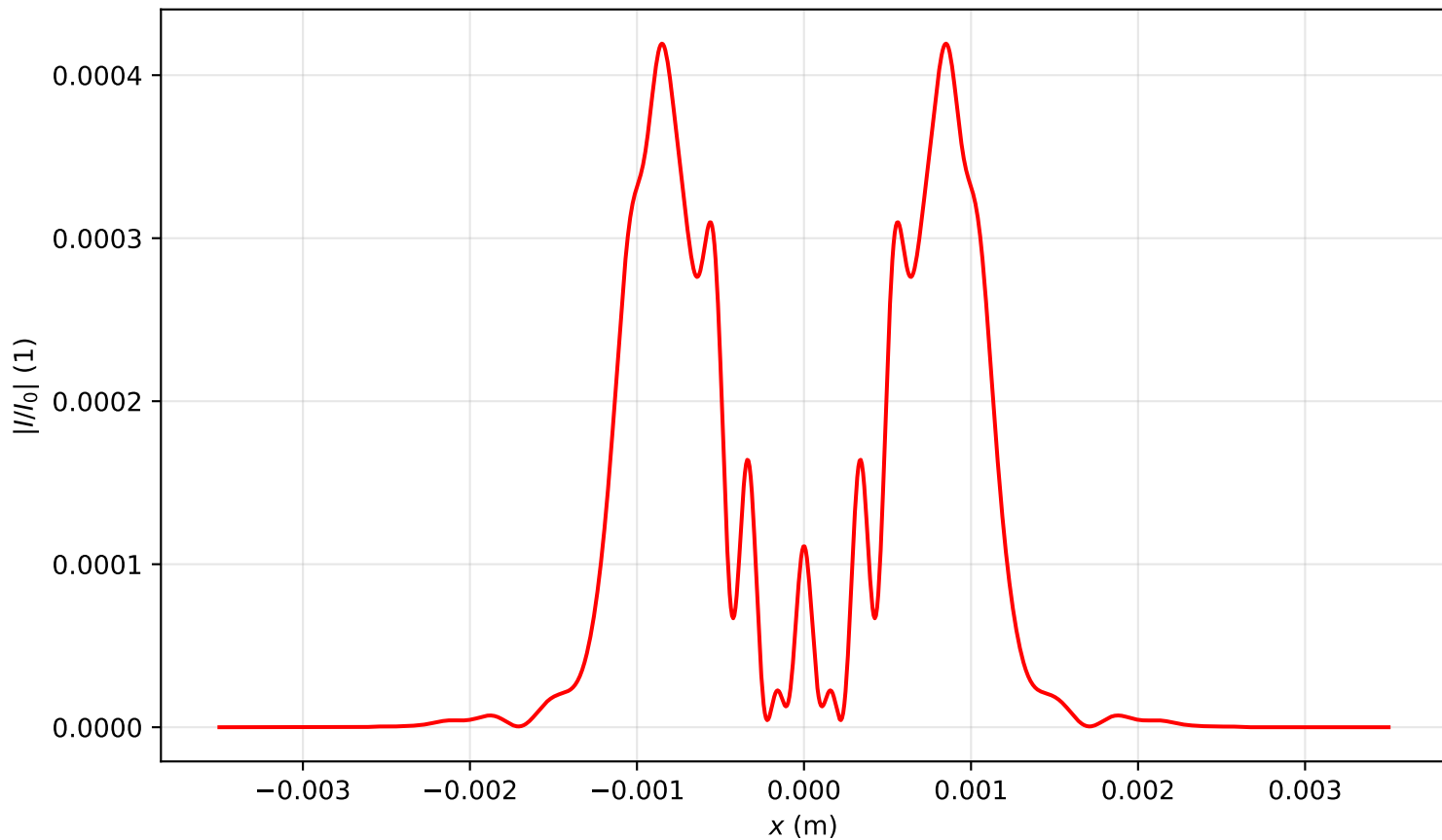
Intensity profile I(x, y = 0, z = 0.876)/I_0 , P_{in}=11.0P_{cr} , artificial time
