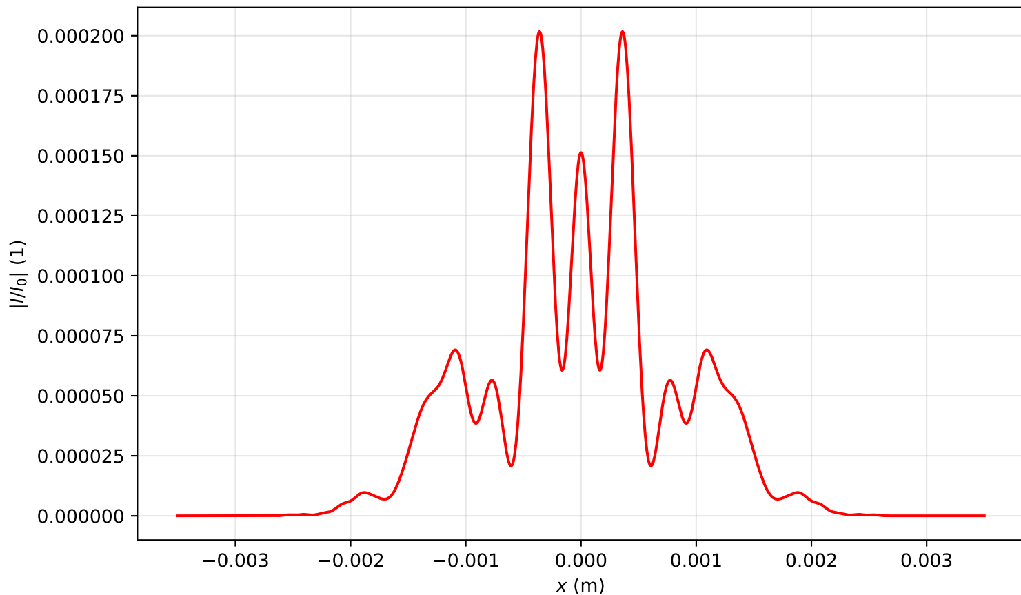
Intensity profile I(x, y = 0, z = 1.194)/I_0 , P_{in}=11.0\text{Pcr} , artificial time
