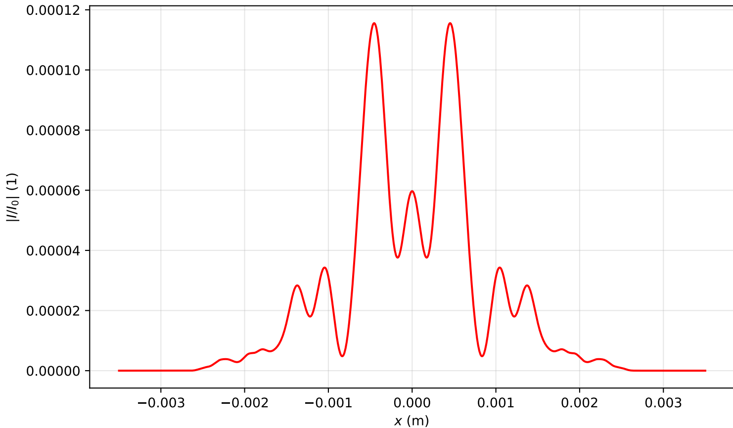
Intensity profile I(x, y = 0, z = 1.353)/I_0 , P_{in}=11.0P_{cr} , artificial time
