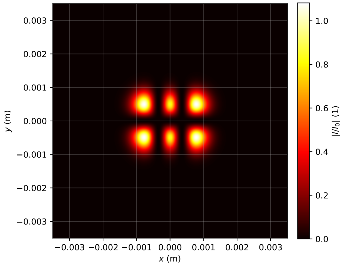
Intensity profile I(x, y, z = 0.080)/I_0 , P_{in}=11.0\text{Pcr} , artificial time
