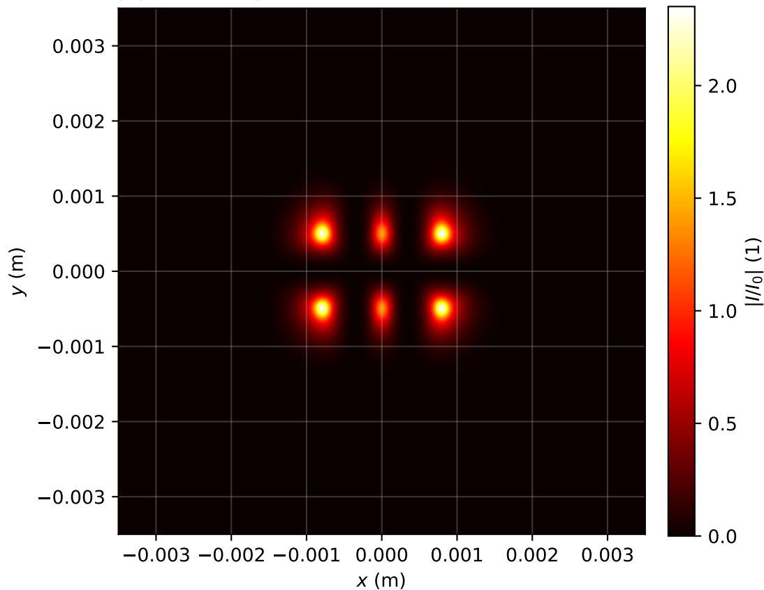
Intensity profile I(x, y, z = 0.239)/I_0 , P_{in}=11.0\text{Pcr} , artificial time
