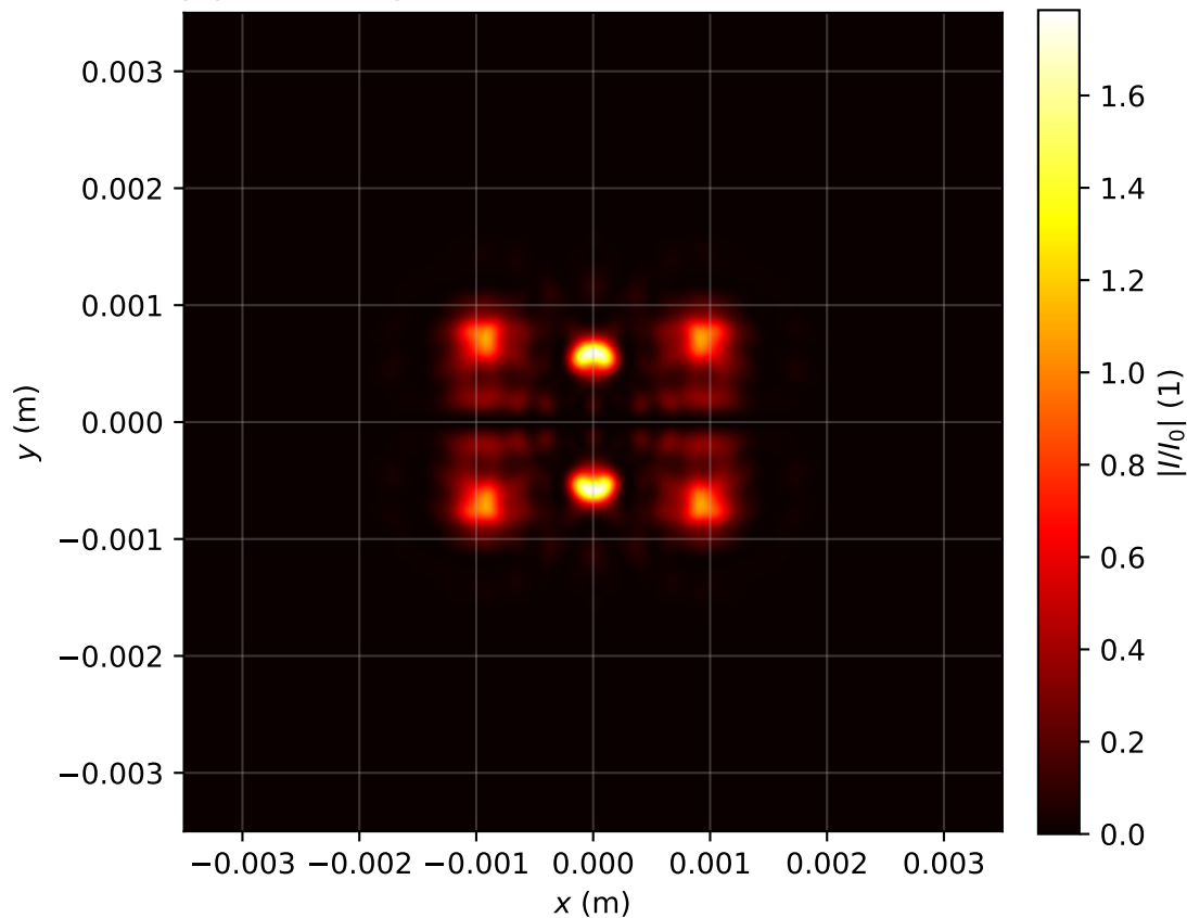
Intensity profile I(x, y, z = 0.955)/I_0 , P_{in}=11.0\text{Pcr} , artificial time
