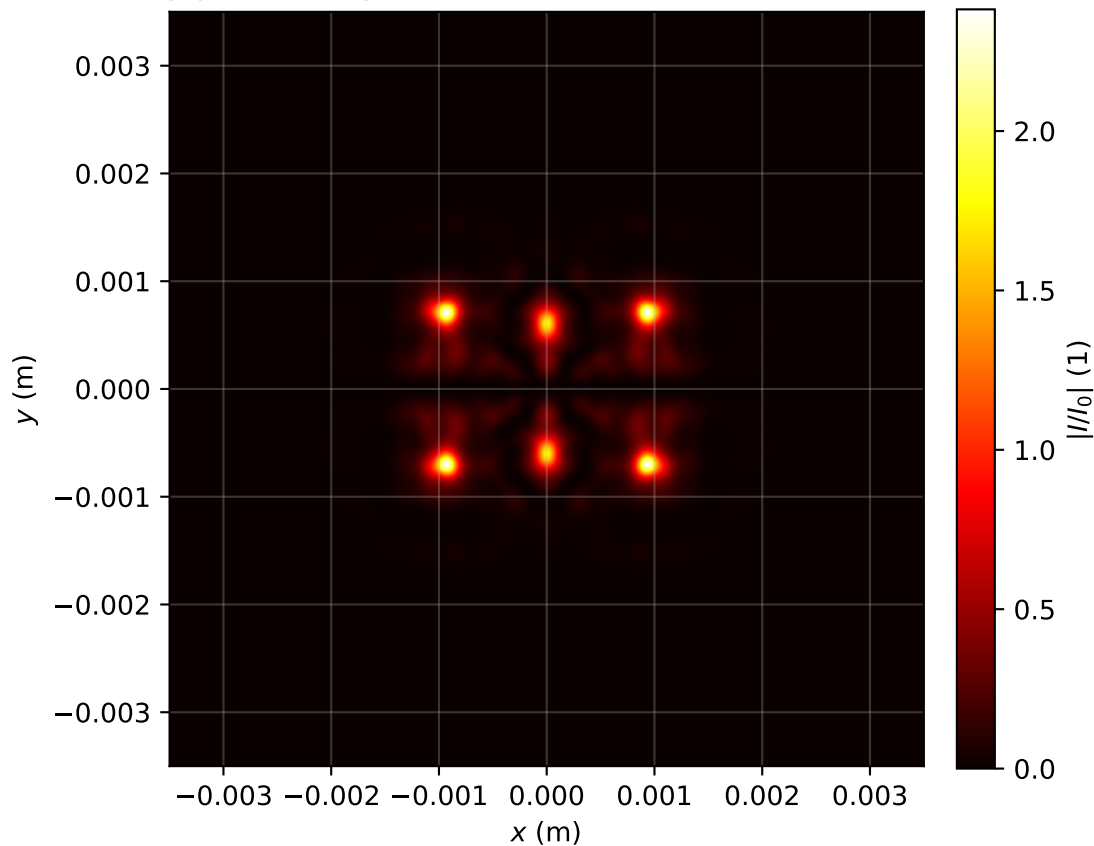
Intensity profile I(x, y, z = 1.115)/I_0 , P_{in}=11.0P_{cr} , artificial time
