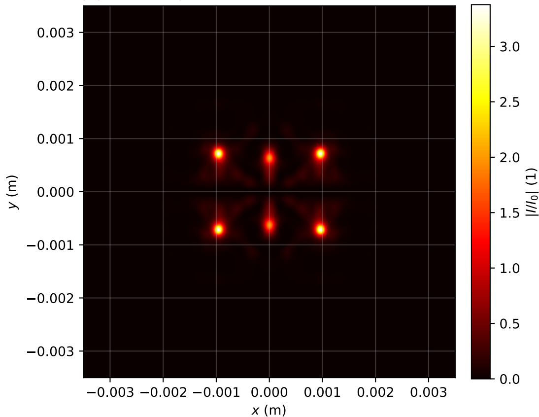
Intensity profile I(x, y, z = 1.194)/I_0 , P_{in}=11.0\text{Pcr} , artificial time
