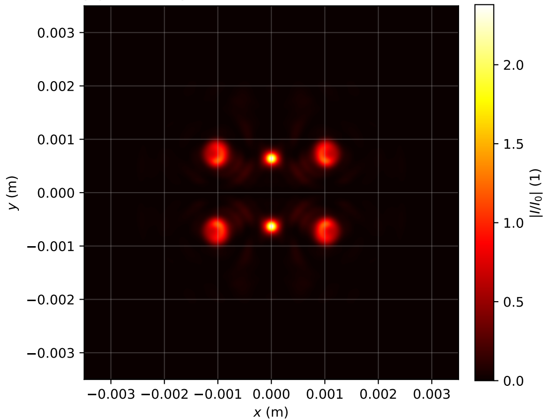
Intensity profile I(x, y, z = 1.592)/I_0 , P_{in}=11.0\text{Pcr} , artificial time
