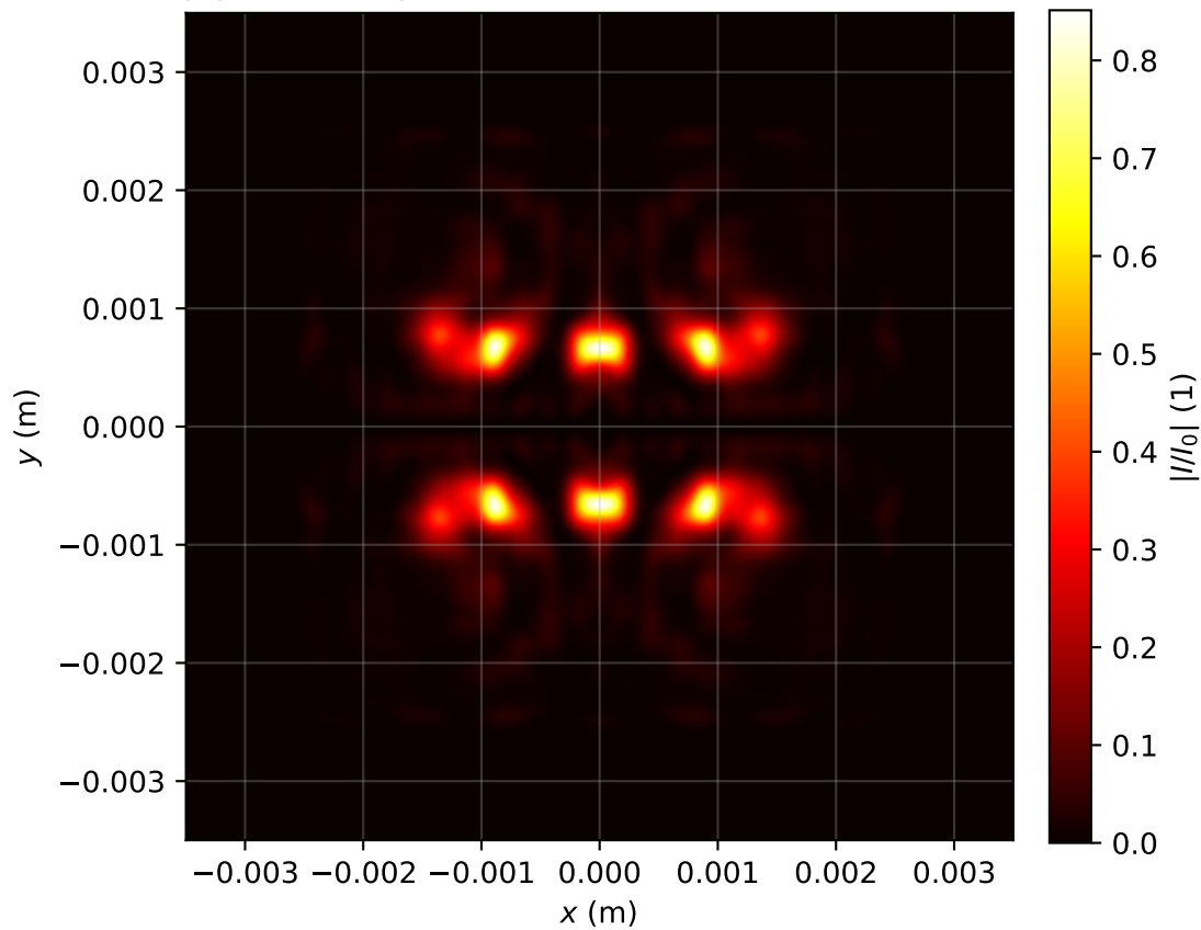
Intensity profile I(x, y, z = 2.070)/I_0 , P_{in}=11.0P_{cr} , artificial time
