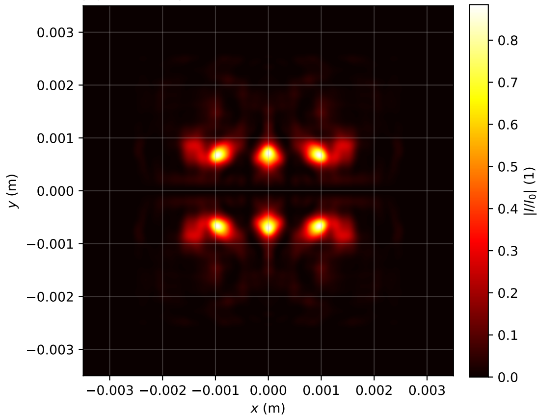
Intensity profile I(x, y, z = 2.149)/I_0 , P_{in}=11.0\text{Pcr} , artificial time
