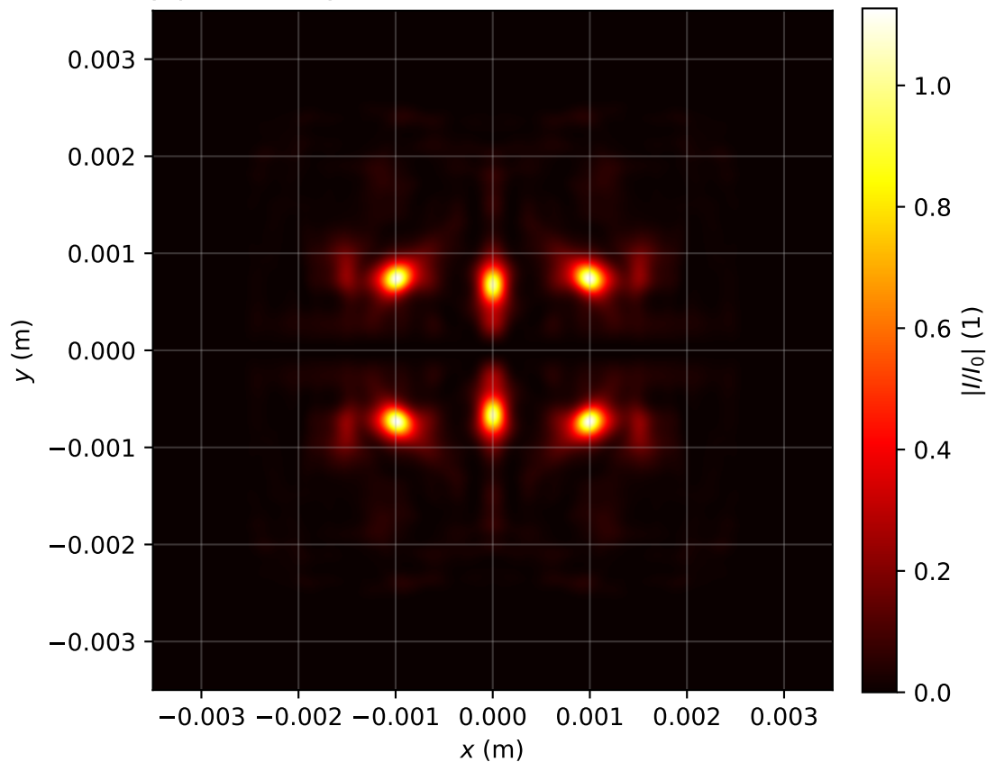
Intensity profile I(x, y, z = 2.309)/I_0 , P_{in}=11.0\text{Pcr} , artificial time
