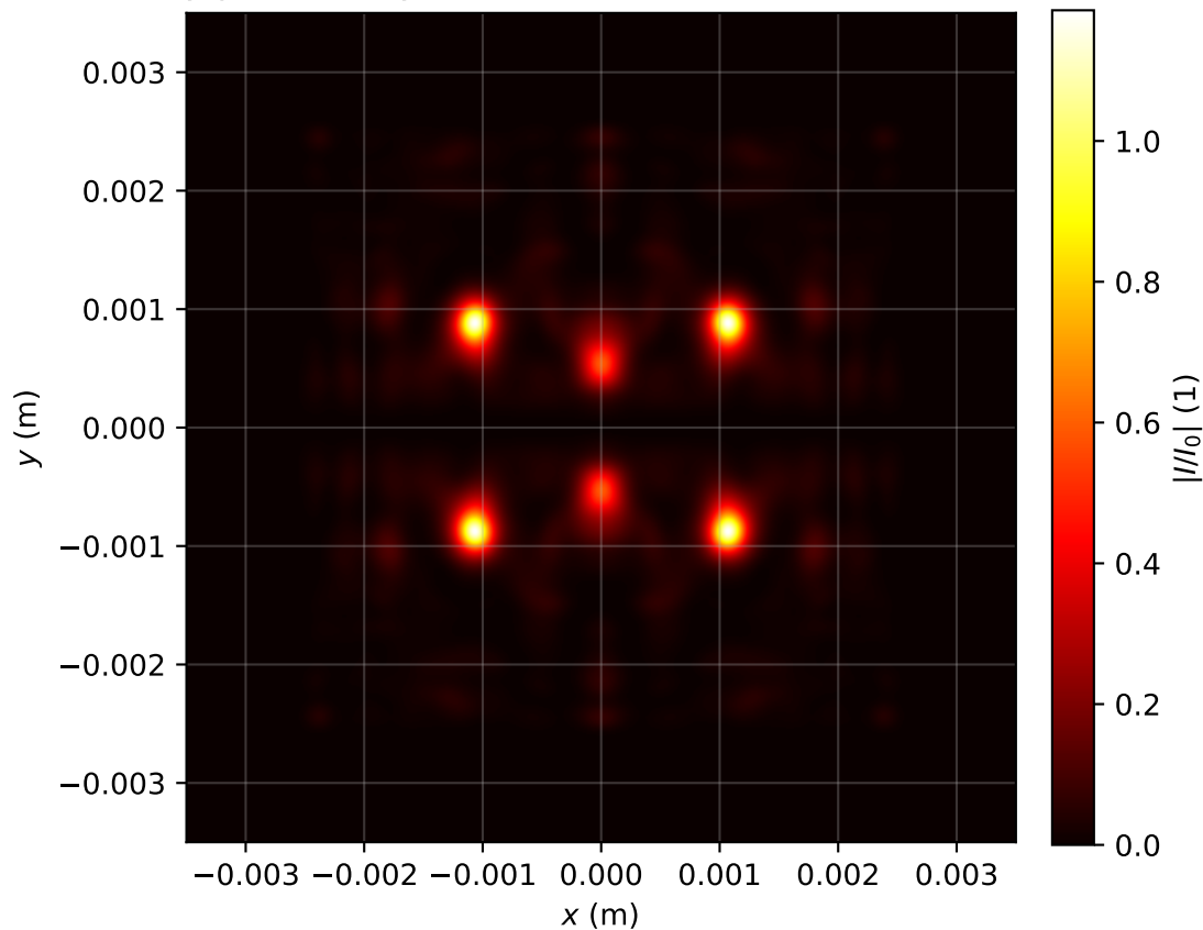
Intensity profile I(x, y, z = 2.707)/I_0 , P_{in}=11.0\text{Pcr} , artificial time
