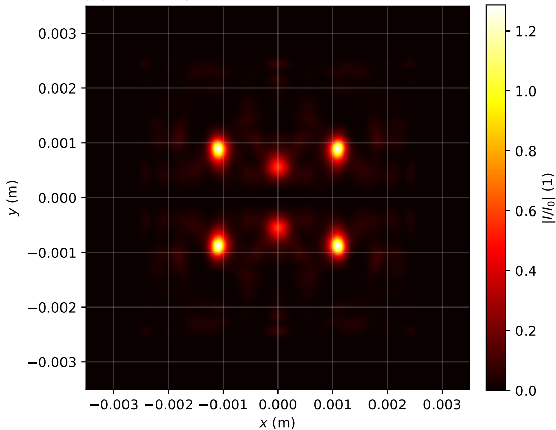
Intensity profile I(x, y, z = 2.786)/I_0 , P_{in}=11.0P_{cr} , artificial time
