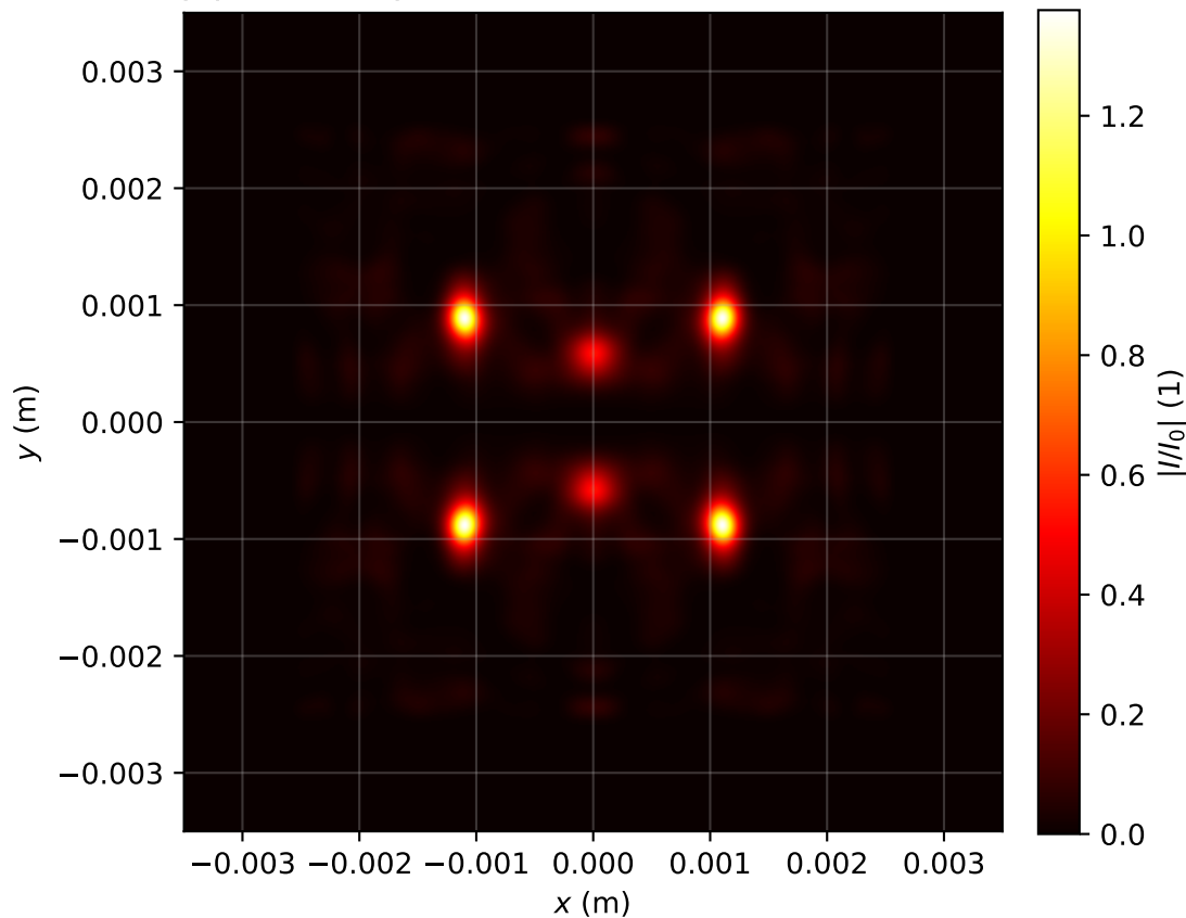
Intensity profile I(x, y, z = 2.866)/I_0 , P_{in}=11.0\text{Pcr} , artificial time
