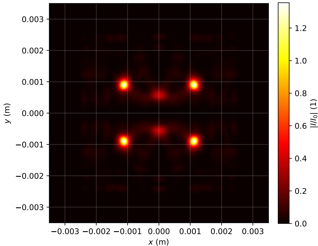
Intensity profile I(x, y, z = 3.025)/I_0 , P_{in}=11.0\text{Pcr} , artificial time
