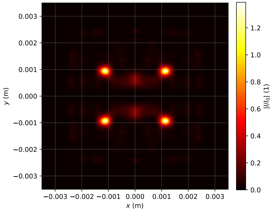
Intensity profile I(x, y, z = 3.184)/I_0 , P_{in}=11.0\text{Pcr} , artificial time
