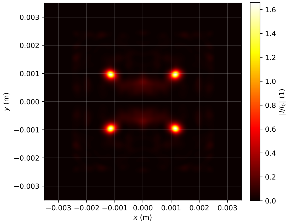
Intensity profile I(x, y, z = 3.344)/I_0 , P_{in}=11.0\text{Pcr} , artificial time
