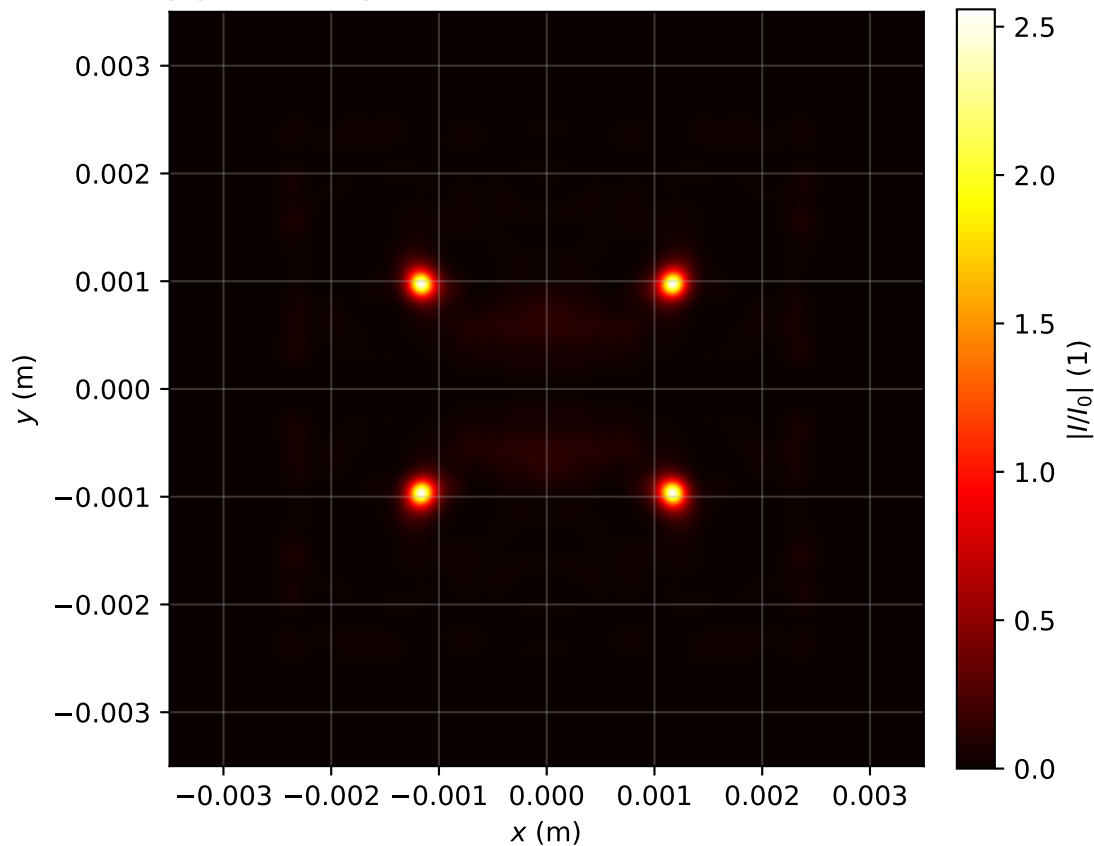
Intensity profile I(x, y, z = 3.503)/I_0 , P_{in}=11.0\text{Pcr} , artificial time
