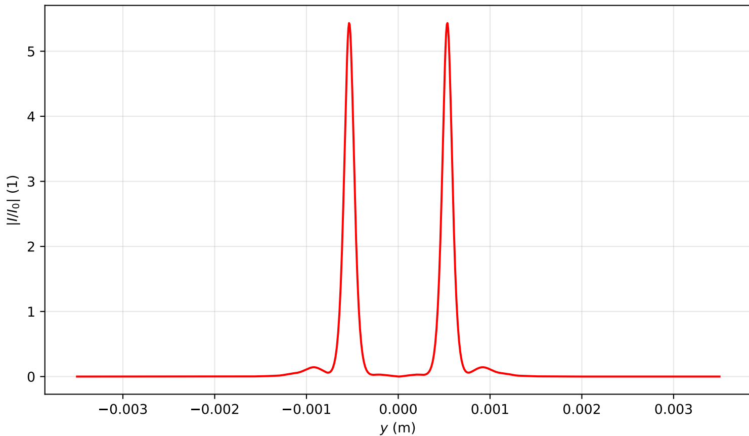
Intensity profile I(x=0, y, z=0.557)/I_0 , P_{in}=11.0\text{Pcr} , artificial time
