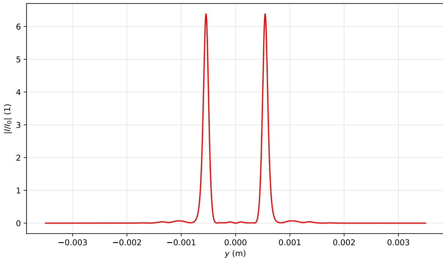
Intensity profile I(x=0, y, z=0.876)/I_0 , P_{in}=11.0P_{cr} , artificial time
