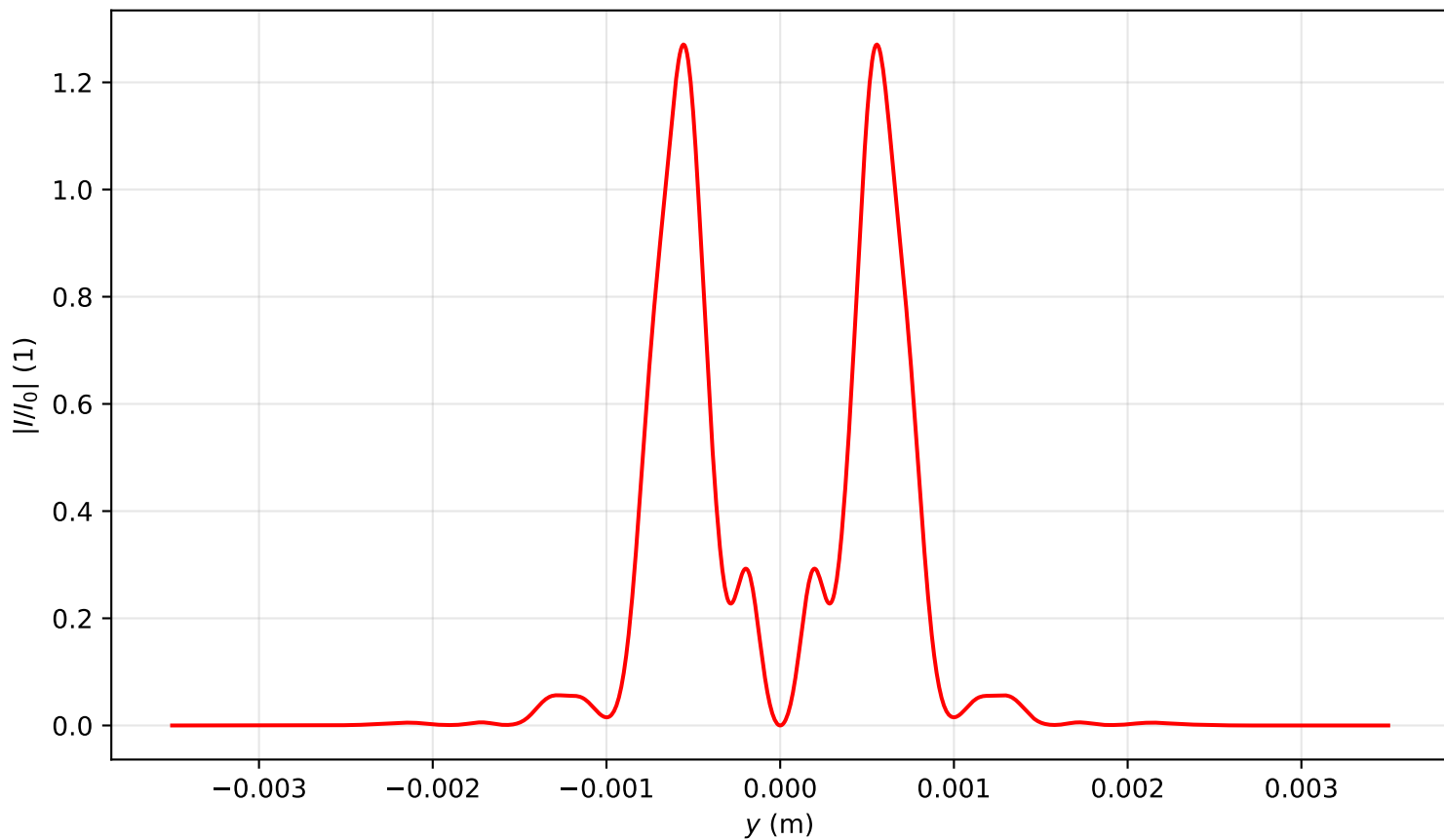
Intensity profile I(x=0, y, z=1.035)/I_0 , P_{in}=11.0P_{cr} , artificial time
