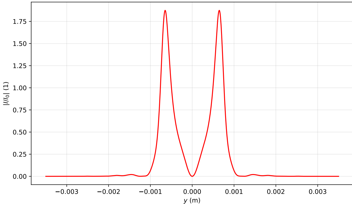
Intensity profile I(x=0, y, z=1.274)/I_0 , P_{in}=11.0P_{cr} , artificial time
